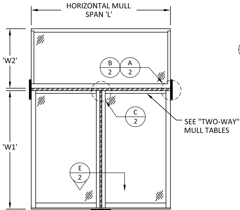
HORIZONTAL "T" MULL SPAN
